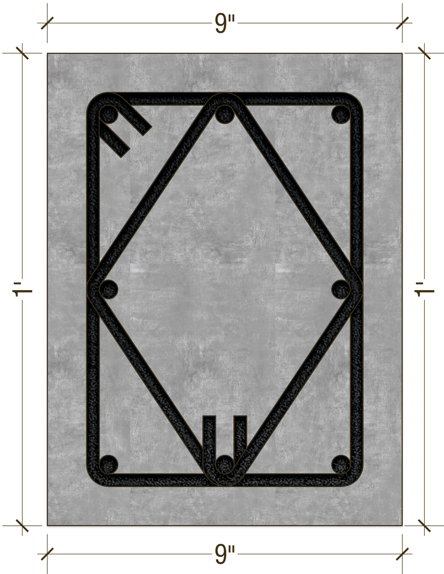
COLUMN DETAILS
